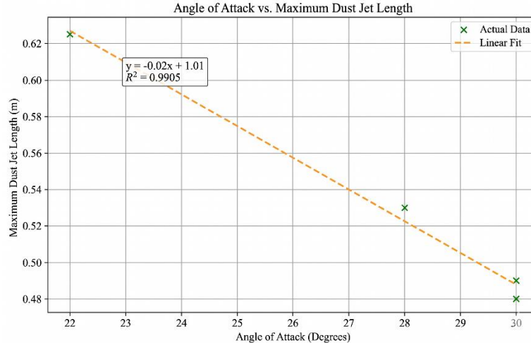
Fig. 23 Angle of attack vs Maximum Dust of Jet Length
