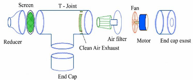
Fig. 16 Exploded view of the fugitive vehicular dust collector.
