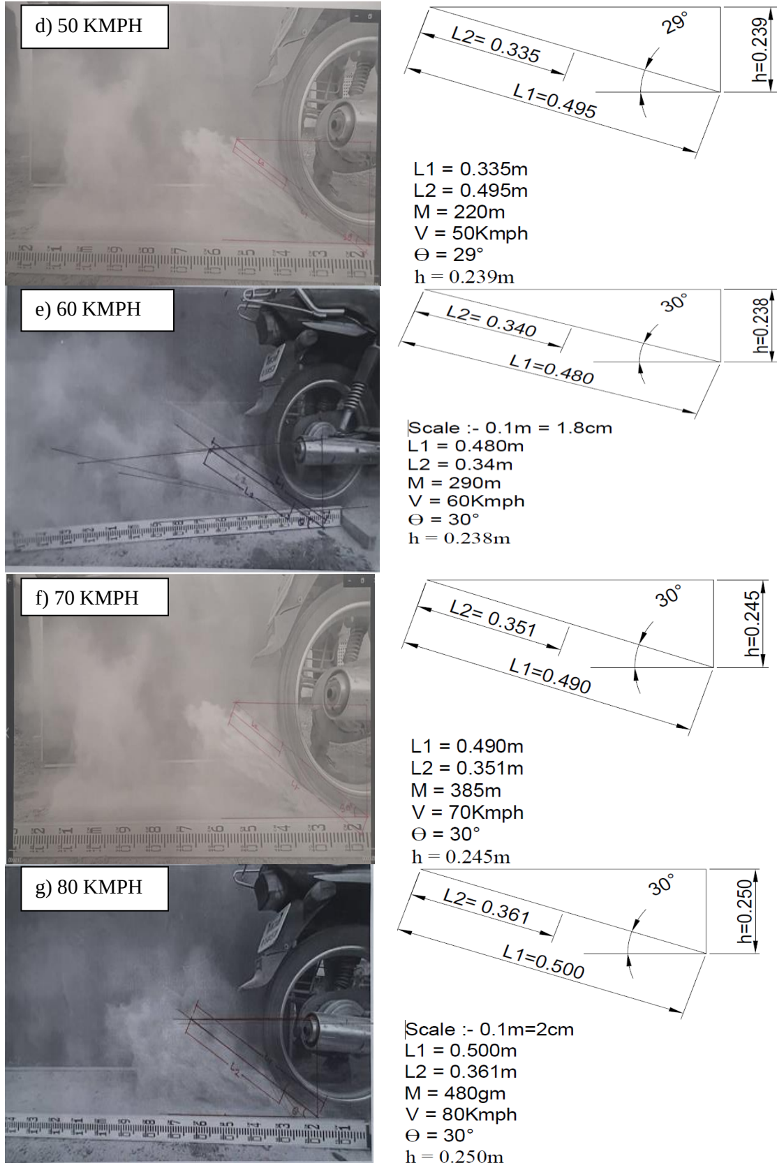
Fig. 20 Investigation for the actual angle of jet coming from the vehicle at different speeds
