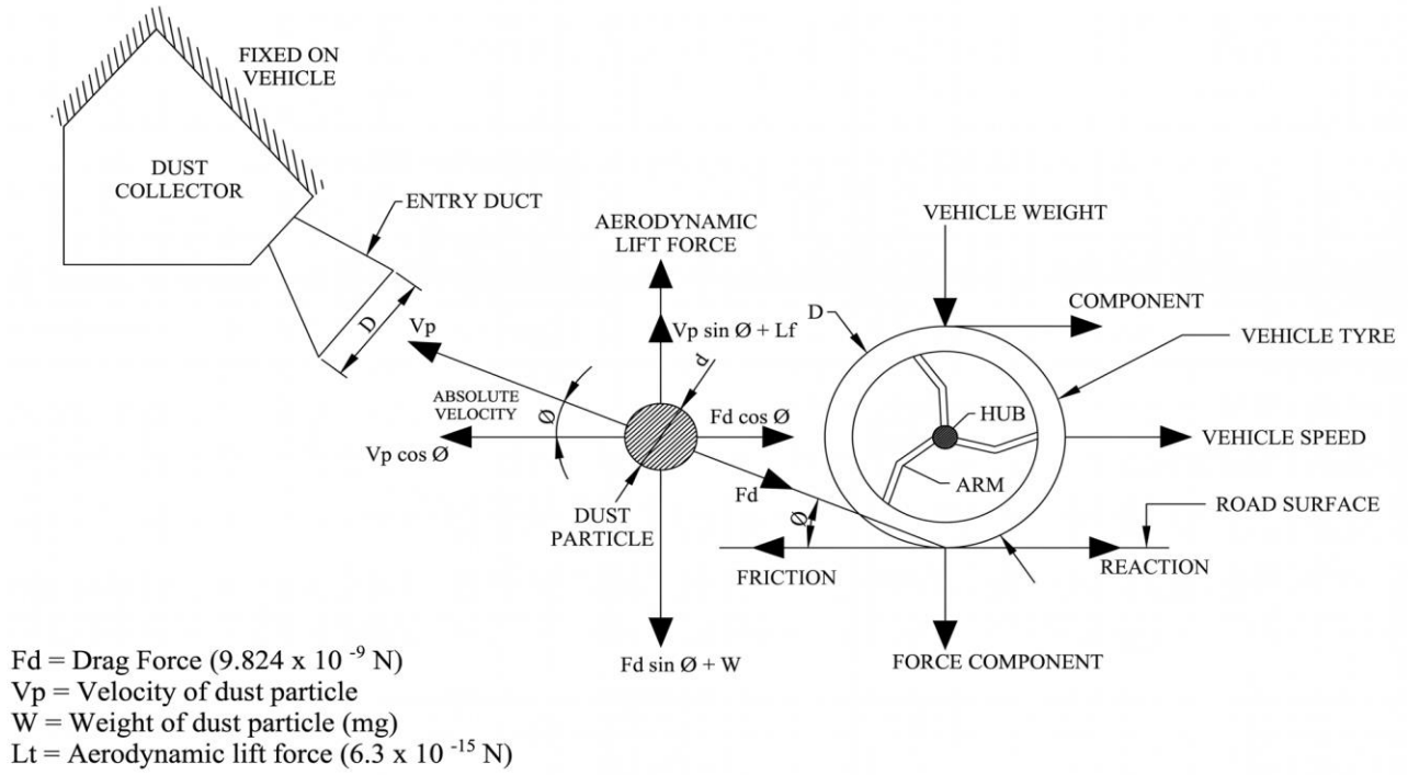
Fig. 13 Drag force on the dust particle
