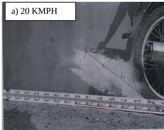
Fig. 19 Investigation for location to mount the prototype on the vehicle (a) Behaviour of Jet (b) Dust collection
