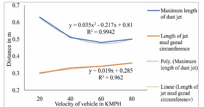
Fig. 26 Length of jet mud guard for 20KMPH
