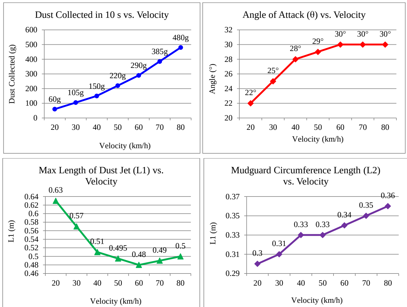
Fig. 24 Correlation between vehicle velocity, mass of collected dust in 10 sec sampling and the resulting dust jet angle of attack
