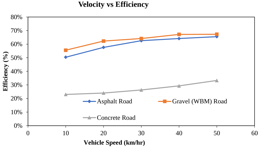
Fig. 30 Velocity vs Efficiency
