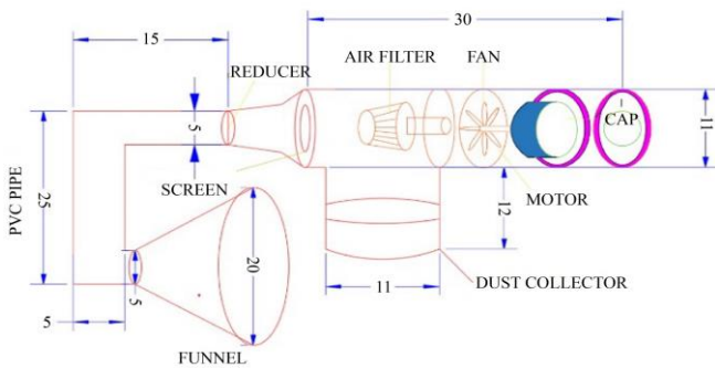
Fig. 15 Fugitive vehicular dust collector
