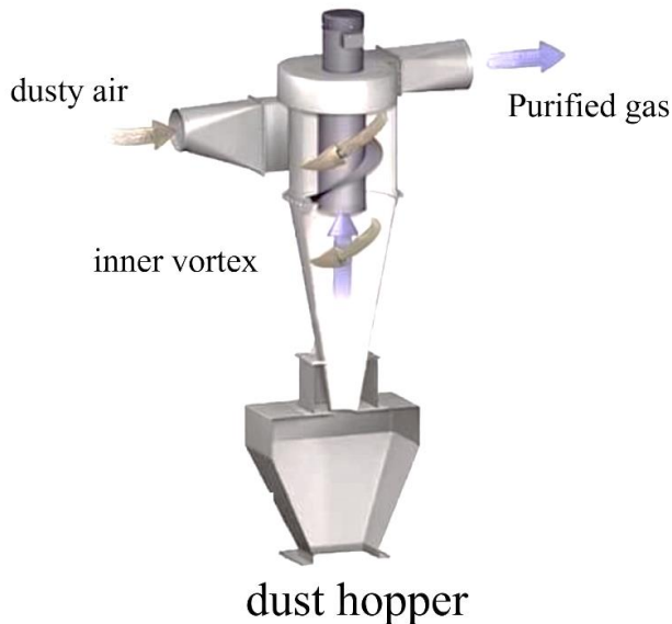
Fig. 7 Cyclone-type road dust collector [37]
