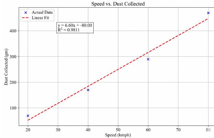
Fig. 22 Speed vs dust collected
