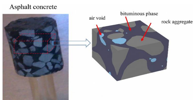
Fig. 4 Material composition of a common asphalt concrete mixture
