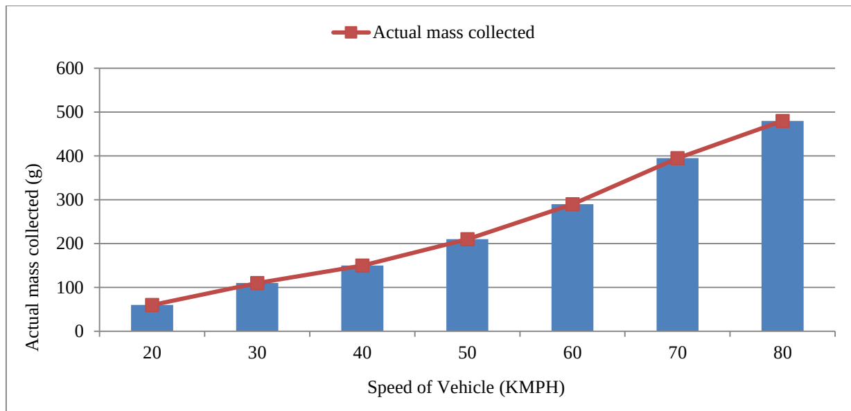
Fig. 21 Vehicle speed vs actual mass collected
