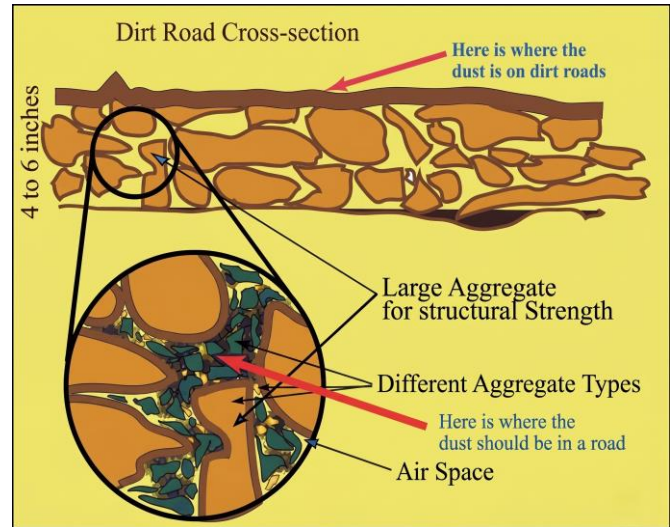
Fig. 2 Mechanism of formation and presence of dust on x-section of WBM road surface [15]
