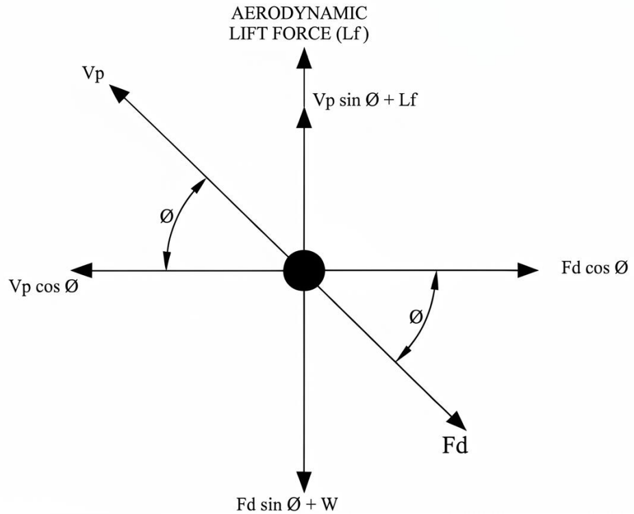
Fig. 13 Drag force on the dust particle
