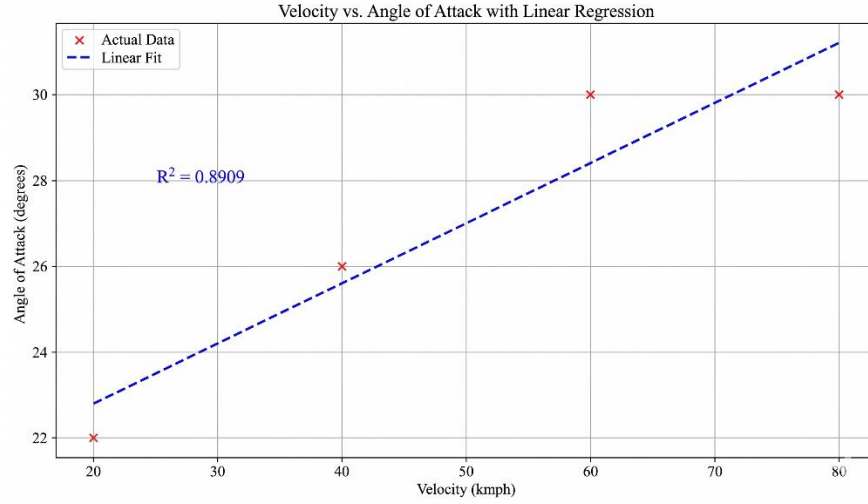
Fig. 25 Angle of attack vs Velocity
