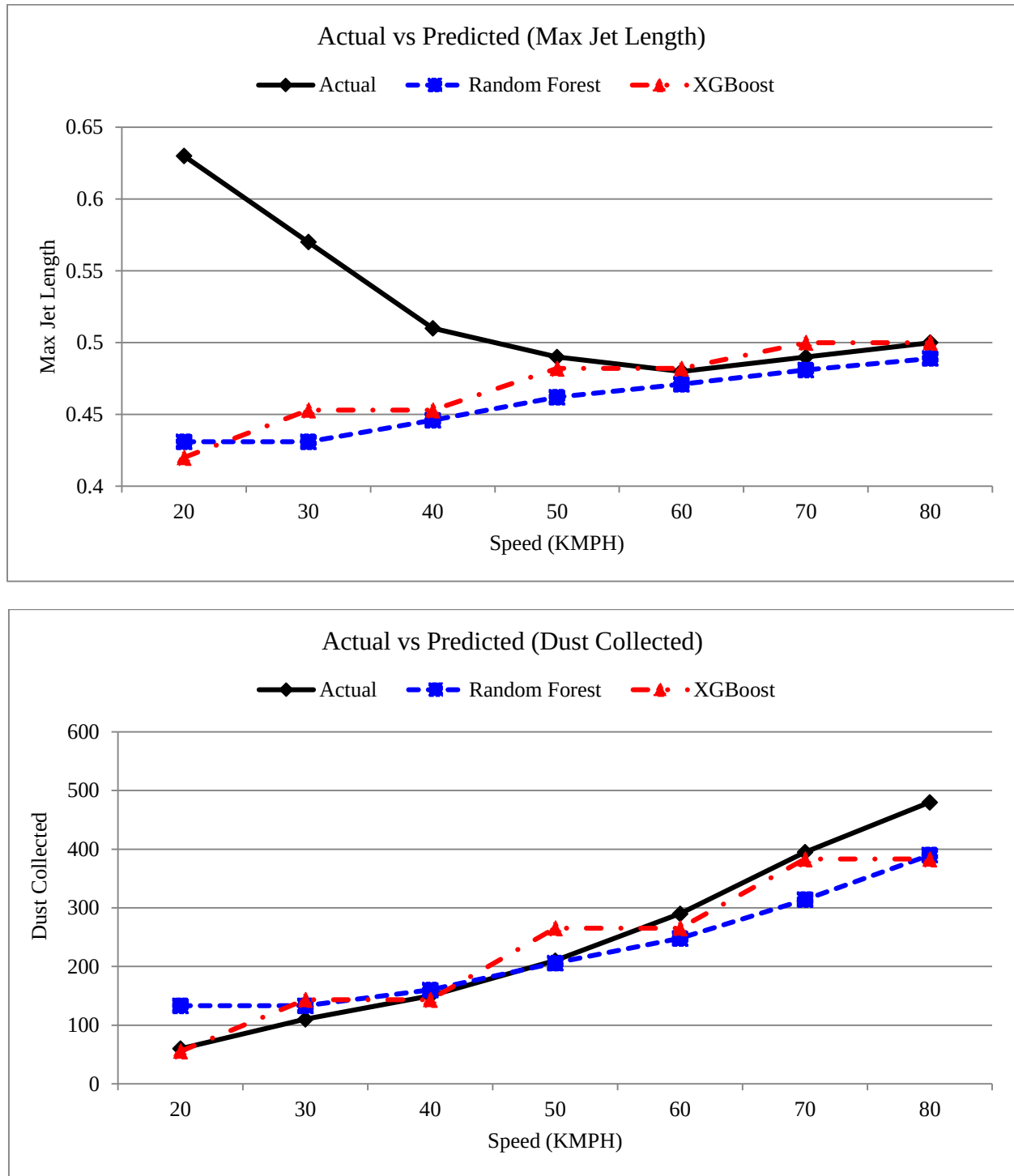
Fig. 27 Model Functioning Pattern of each parameter (Angle of Attack, Dust Collected, and Max Jet Length) with Random Forest (RF) and XGBoost (XGB)
