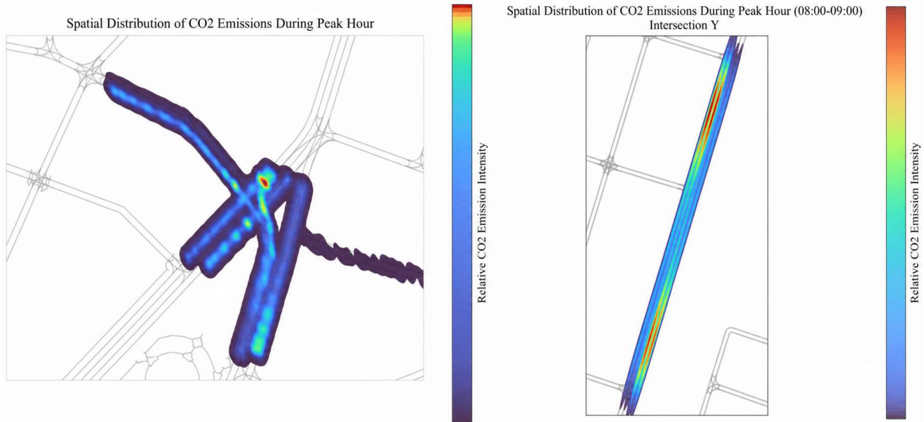
Fig. 18 Spatial distribution of $CO_2$ emissions during peak hours at the studied locations. (a) Location 1 (Signalized intersection context) and Location 2 (Intersection Y). The heatmaps represent the relative $CO_2$ emission intensity based on the spatial data generated by SUMO.
