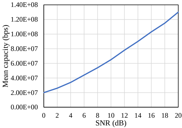
Fig. 2 Monte Carlo simulation of channel capacity
