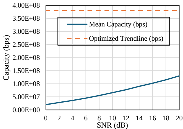
Fig. 6 Channel capacity and channel gain using PSO
