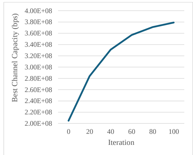
Fig. 7 PSO convergence behavior for channel-capacity optimization
