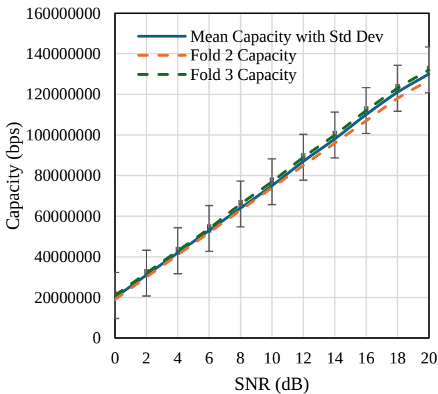
Fig. 3 Monte Carlo simulation with k-fold cross-validation
