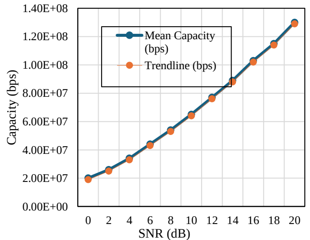
Fig. 4 Trend analysis of channel capacity
