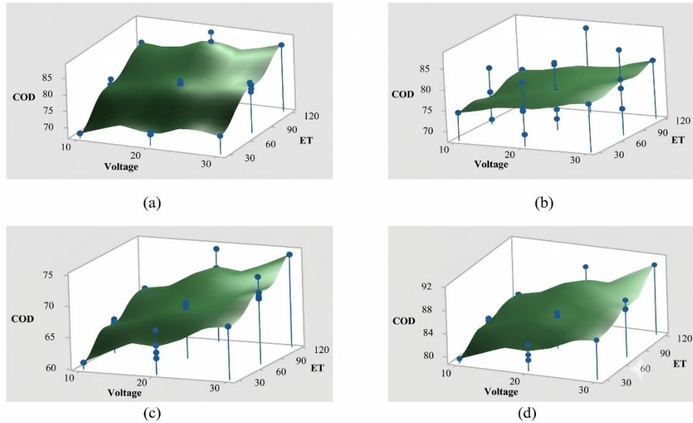
Fig. 3 Electrochemical treatment methods using Fe-Fe electrodes: (a) EC (punched), (b) EC (mesh), (c) AEC (punched), and (d) AEC (mesh) response surfaces and comparison graphs showing COD removal effectiveness.
