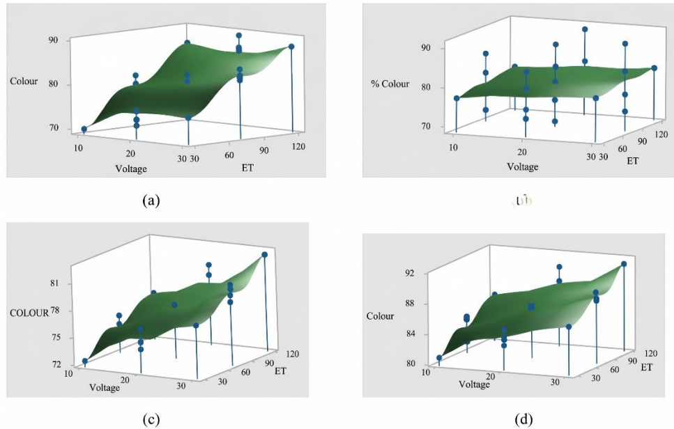
Fig. 2 Electrochemical treatment methods using Fe–Fe electrodes, (a) EC (punched), (b) EC (mesh), (c) AEC (punched), and (d) AEC (mesh) response surfaces and comparison graphs showing color removal effectiveness.
