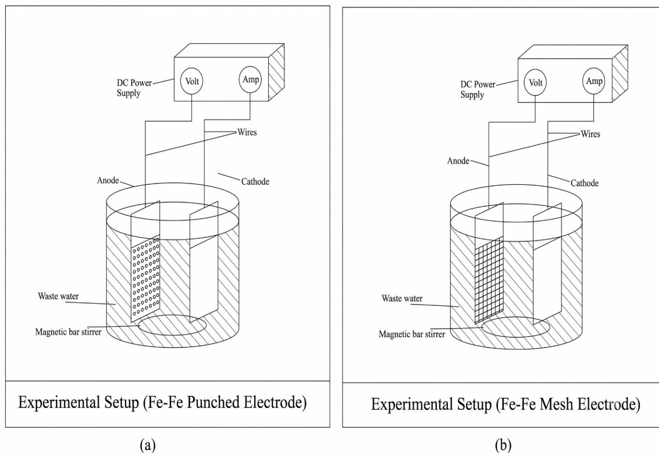
Fig. 1 Experimental setup, (a) Punched electrode, and (b) Mesh electrode.
