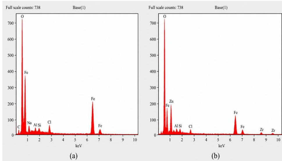
Fig. 6 EDX spectra of Iron electrode (a) Before treatment, and (b) After treatment.
