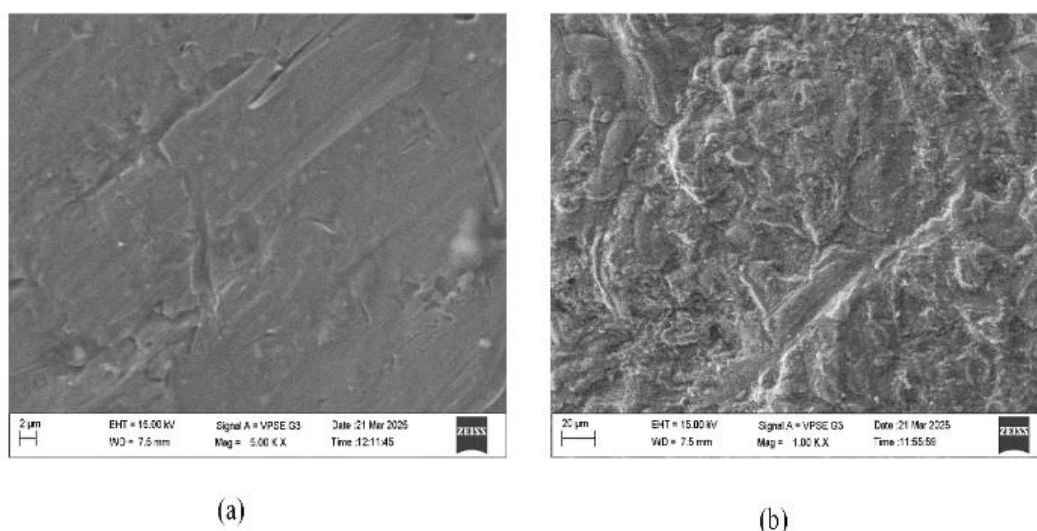
Fig. 5 SEM analysis of Iron electrode (a) SEM analysis of electrode before treatment, and (b) SEM analysis of Electrode after treatment.
