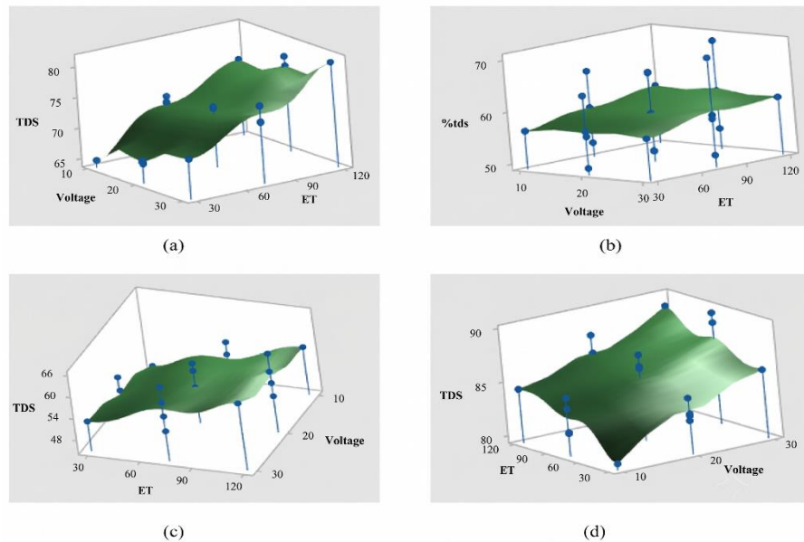
Fig. 4 Electrochemical treatment methods using Fe–Fe electrodes: (a) EC (punched), (b) EC (mesh), (c) AEC (punched), and (d) AEC (mesh) response surfaces and comparison graphs showing TDS removal effectiveness.
