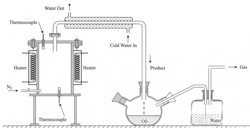
Fig. 1 Schematic diagram of the pyrolysis unit
