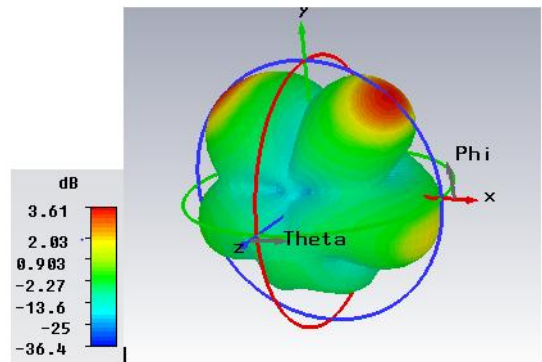
Figure 7. Three dimension radiation pattern of proposed UWB antenna.
