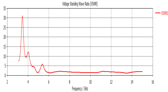
Figure3. Variation of VSWR with frequency UWB antenna.
