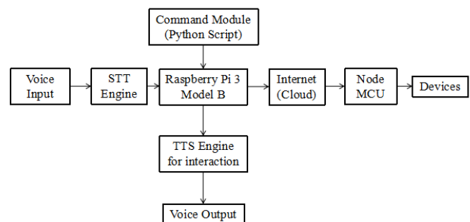
Fig.3 - Architecture
