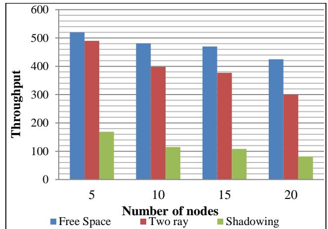
Fig. 6 Throughput comparison
