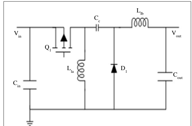
Fig. 3 Zeta converter's equivalent circuit
