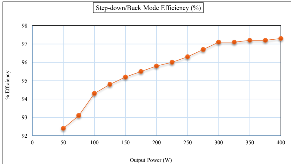
Fig. 19 Efficiency of the presented converter in both modes
