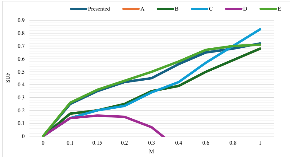
Fig. 18 Comparison of Semiconductor Utilization Factor (SUF) w.r.t Voltage Gain (M) for Buck Mode {Reference A-(17); B-(13); C-(25); D-(21); E-(23)}
